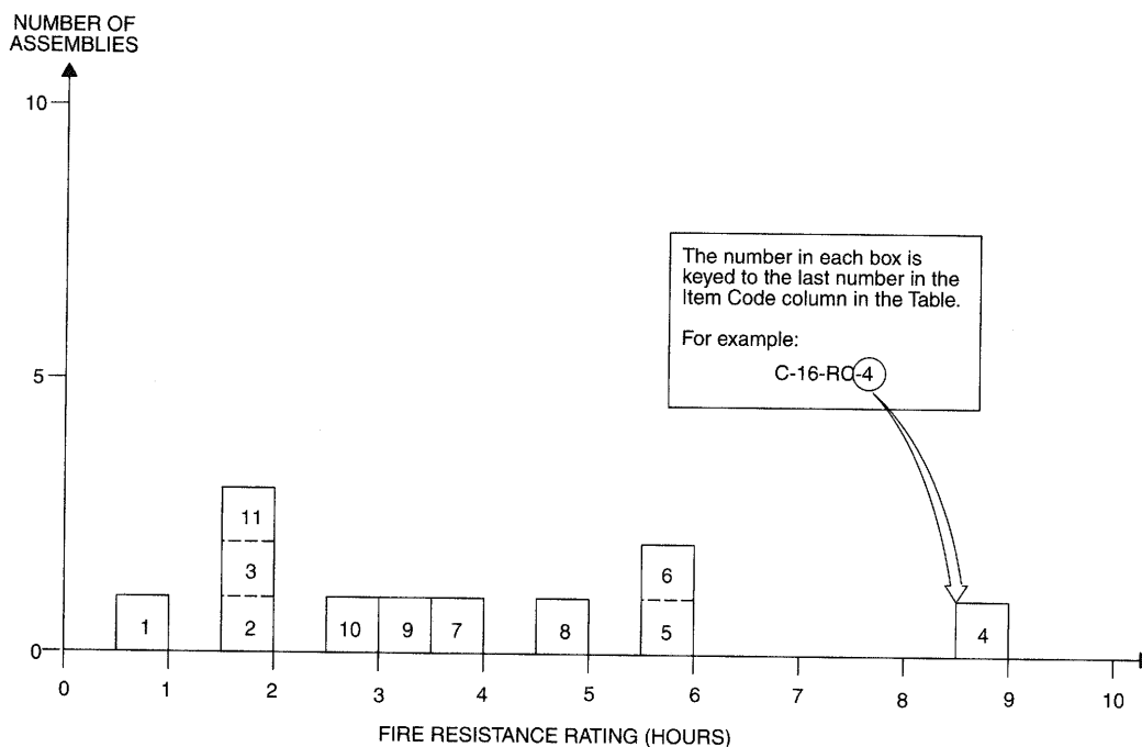
FIGURE 2.1.5—REINFORCED CONCRETE COLUMNS MINIMUM DIMENSION 16" TO LESS THAN 18"
